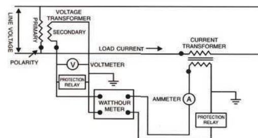
General Application Diagram
